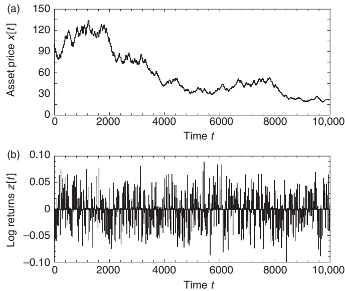
Fig. 5.2 (a) Price and (b) log-returns as a function of time, generated using the EZ model with N = 10,000 agents, \nu = 0.01 and a market depth of \lambda = 5 \times 10^4 .
