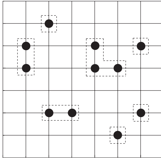
Fig. 5.5 Schematic diagram showing cluster formation on a 2D lattice. Dots represent agents and the dashed lines grouping these agents represent the extent of clusters.
